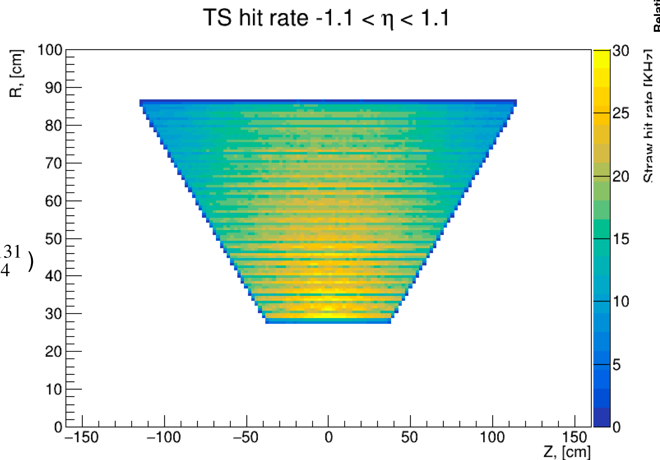
Fig. 19 - TS full hit rate in the central pseudorapidity region for the Xe-Xe collisions
