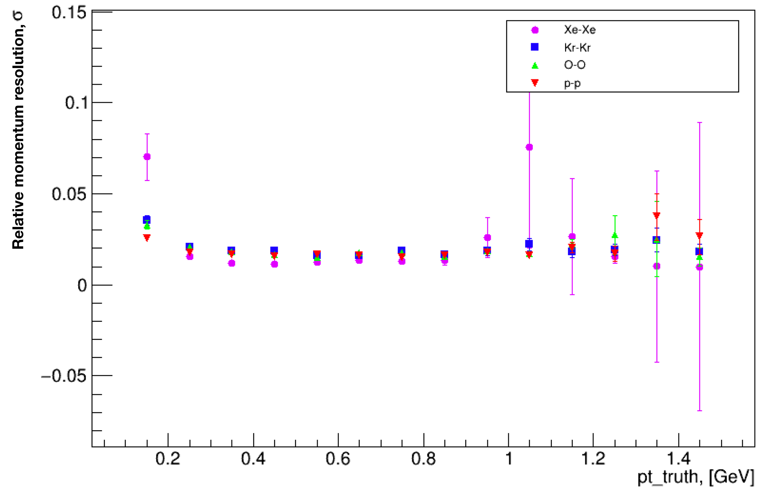
Fig. 21 - Comparison of momentum resolution in the Straw Tracker in p-p and ion-ion collisions
