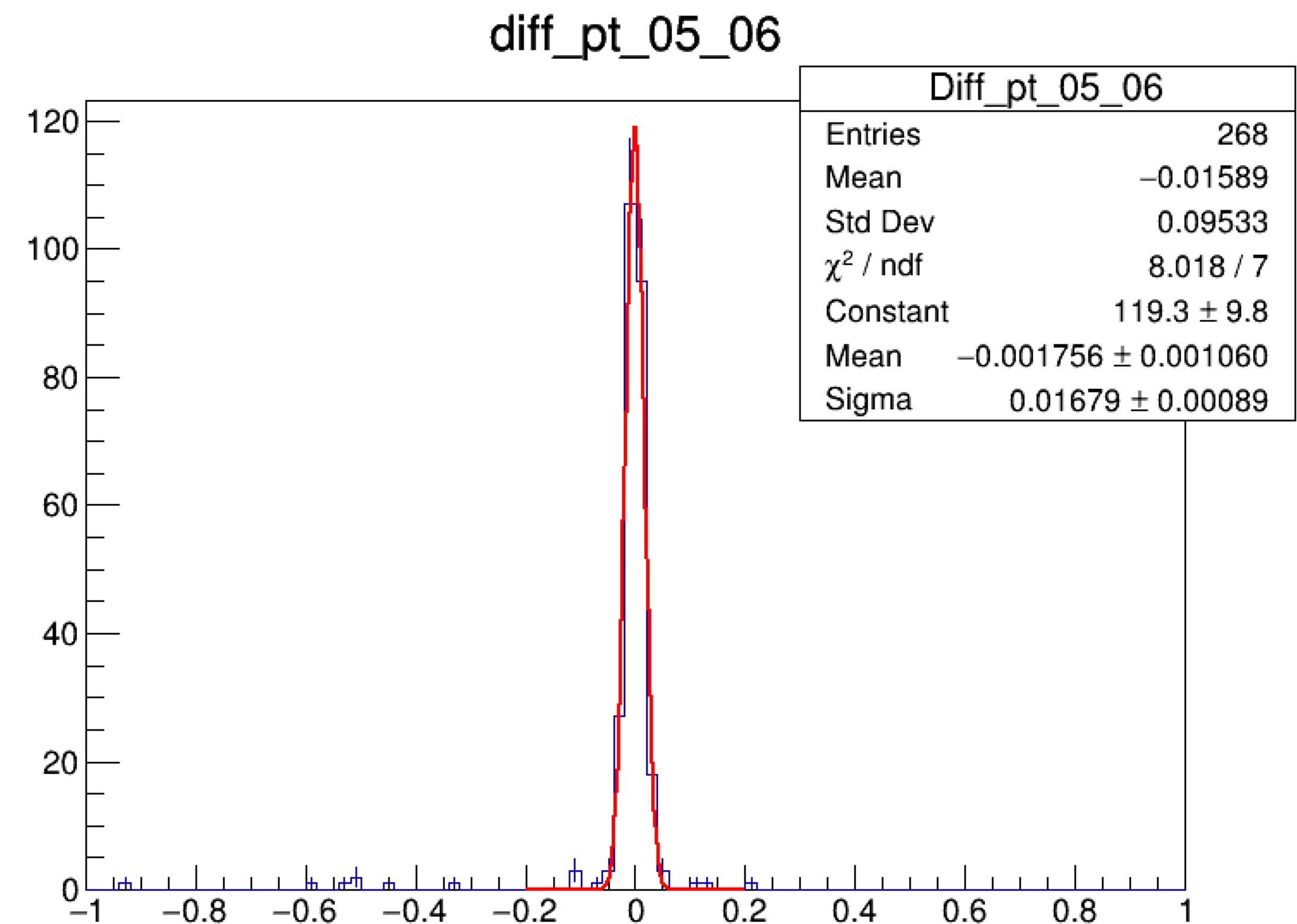
Fig. 34 - Fit results for momentum reconstruction accuracy calculations
