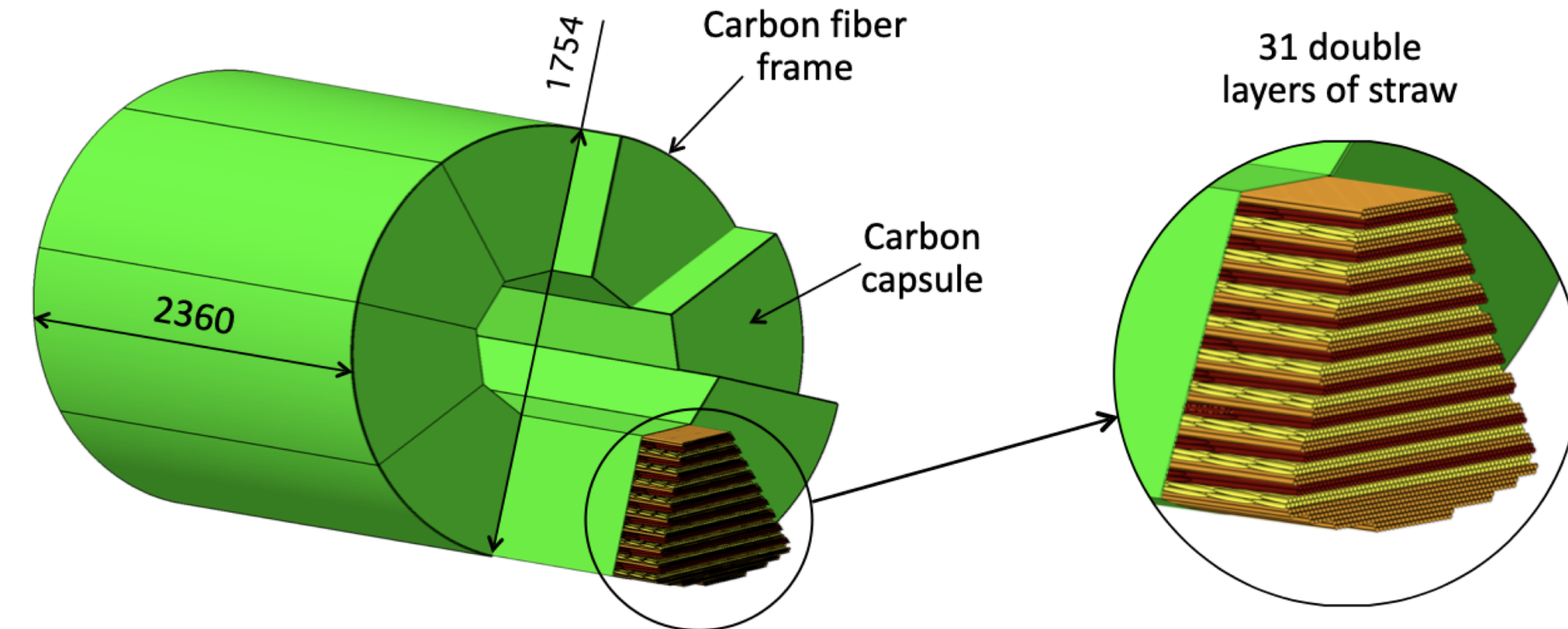
Fig. 3 - Straw Tracker (barrel)
