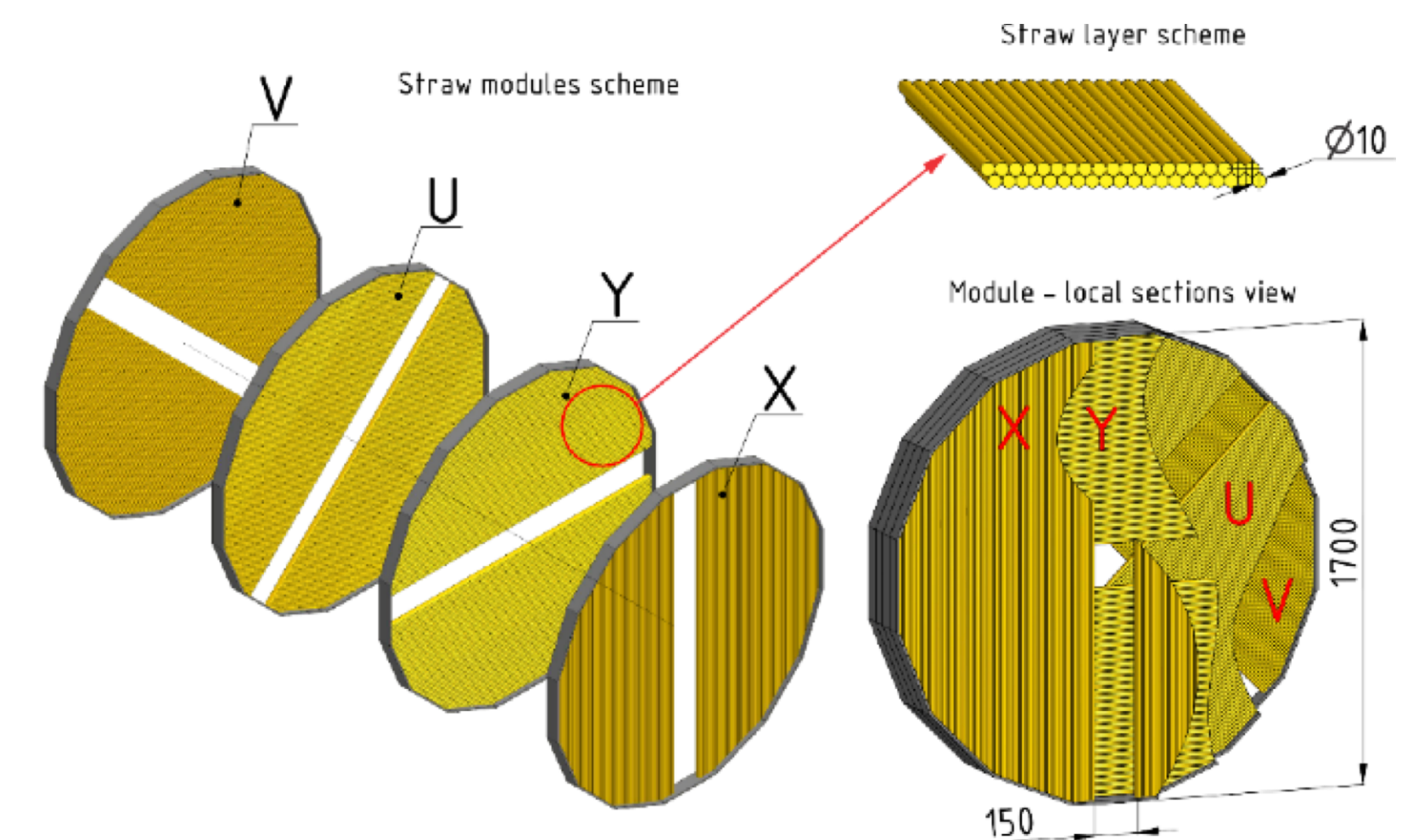
Fig. 4 - Straw Tracker (end-cap)
