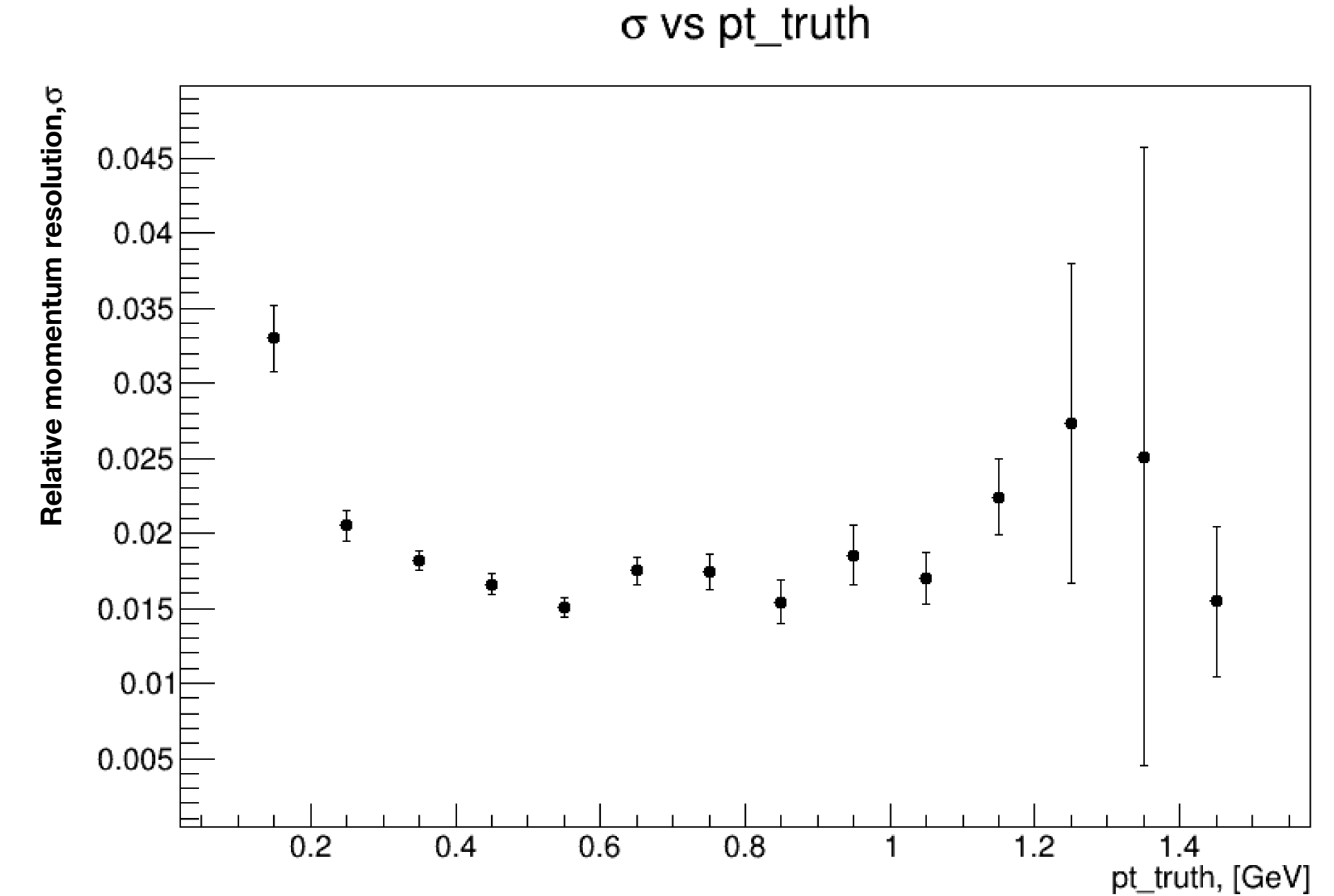
Fig. 12 - Momentum resolution of the Straw Tracker for MC Pt within the central pseudorapidity interval for the O-O collisions
