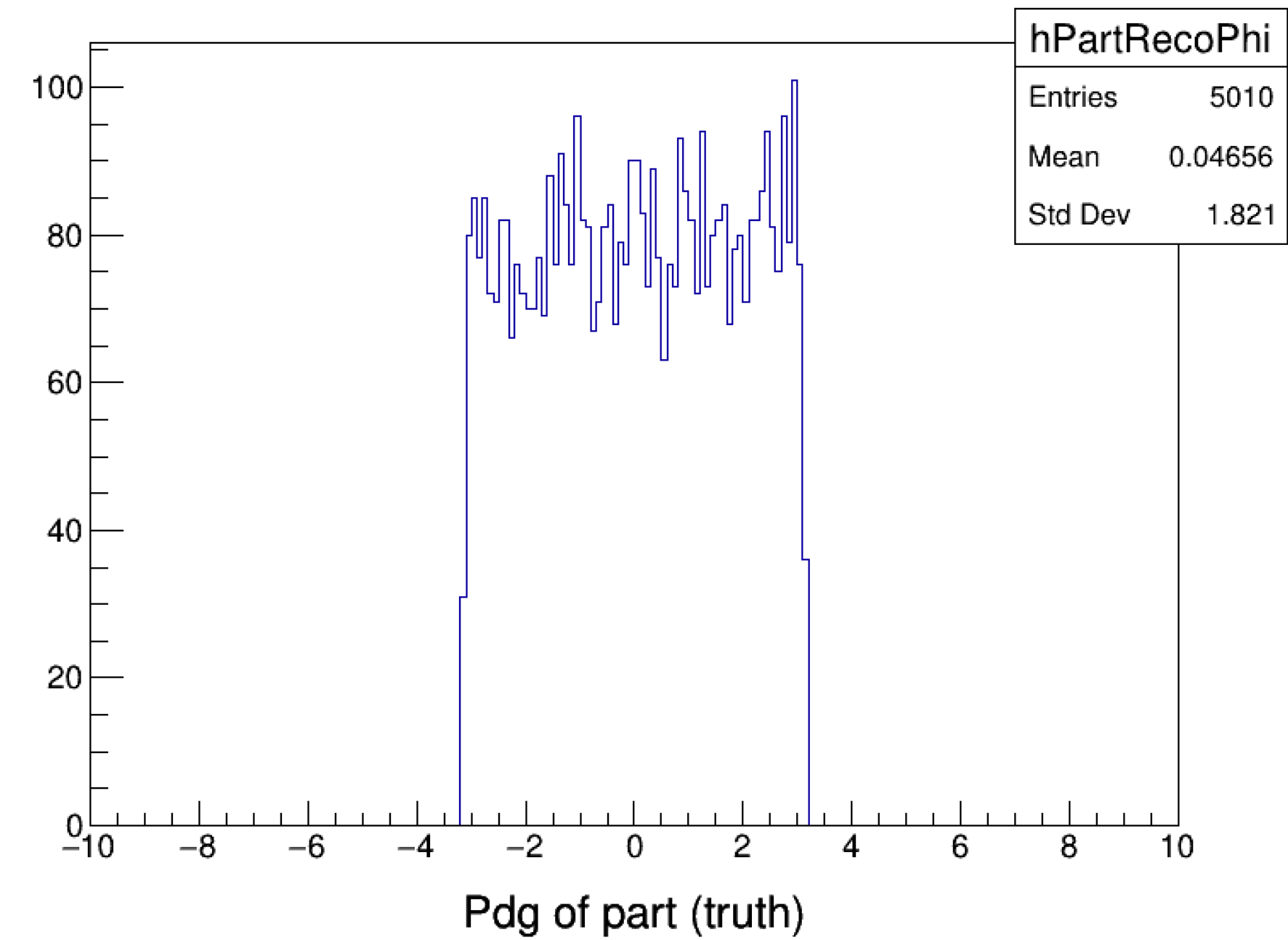
Fig. 36 - Particles parameters from the reconstruction
