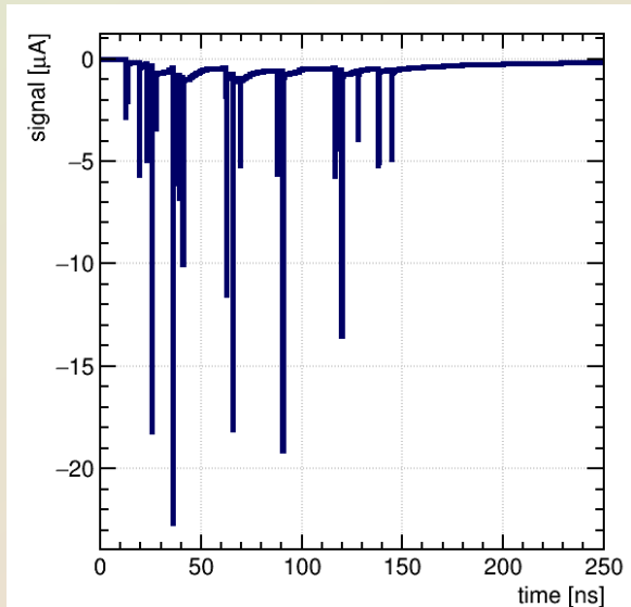
a) Signal from straw tube simulated by Garfield++
