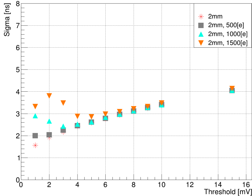
Sigma vs Threshold
