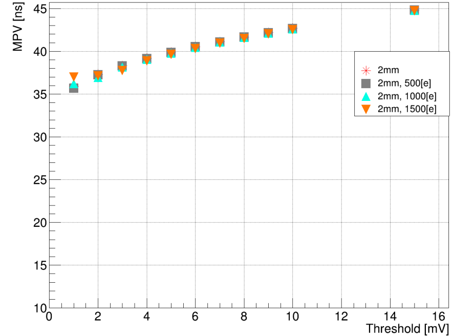
MPV vs Threshold
