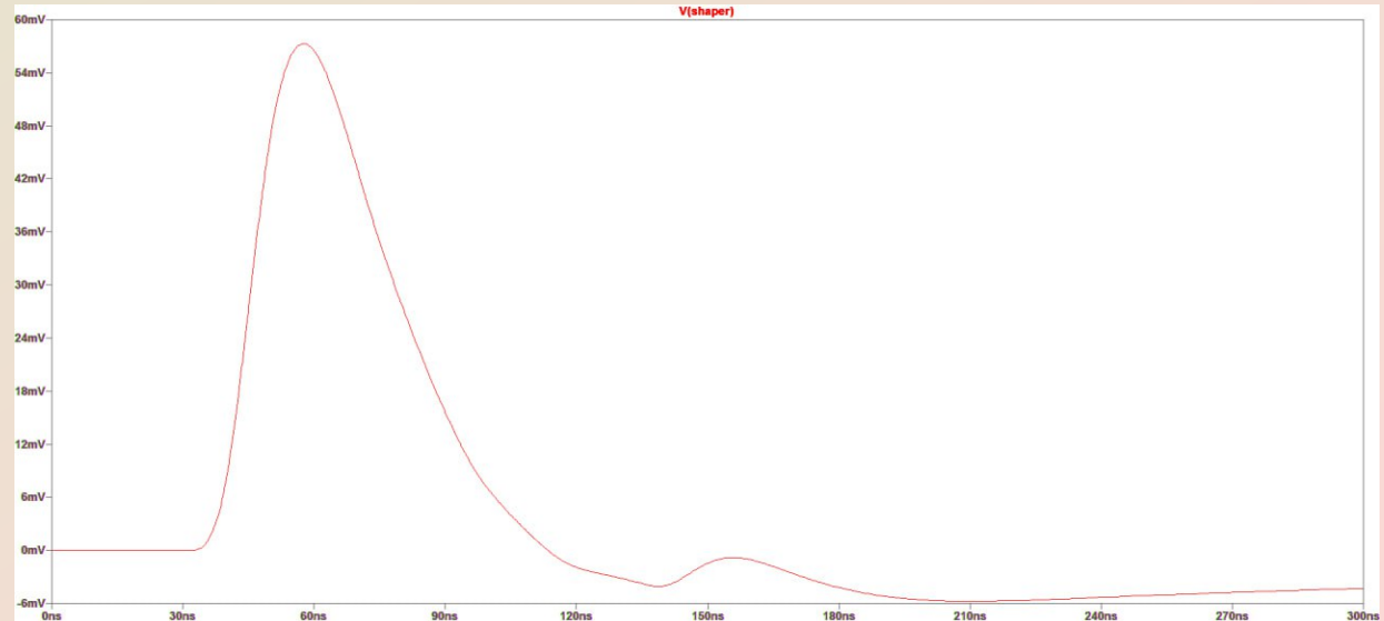
b) LTSpice response to the signal provided by Garfield++
