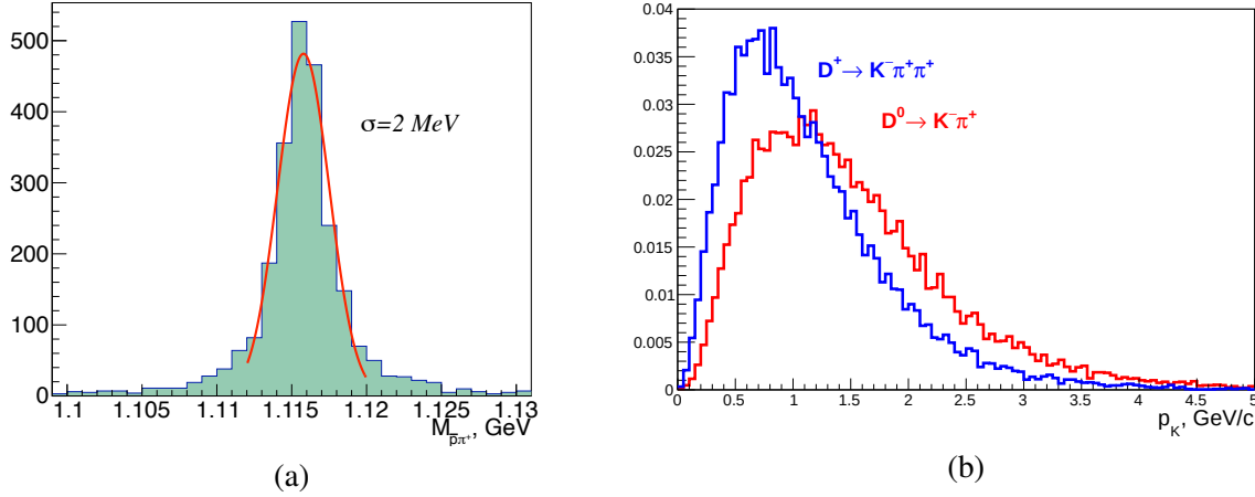
Figure 9.8: (a) \Lambda peak in the p\pi mass spectrum. (b) Kaon spectra from the decays D^0 \rightarrow K^- \pi^+ (red) and D^+ \rightarrow K^- \pi^+ \pi^+ (blue) produced at \sqrt{s} = 27 GeV/c.
