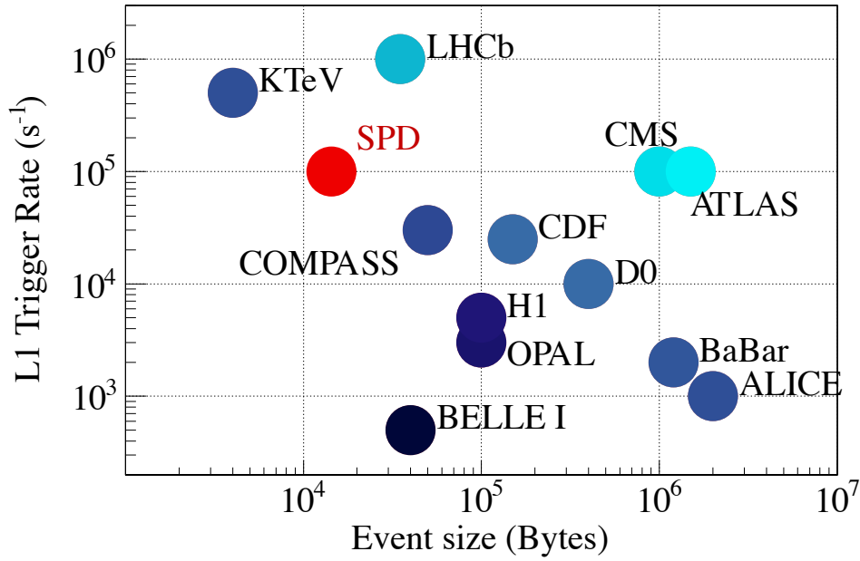
Figure 8.1: Expected event size and event rate of the SPD setup after the online filter compared with other experiments [456].
