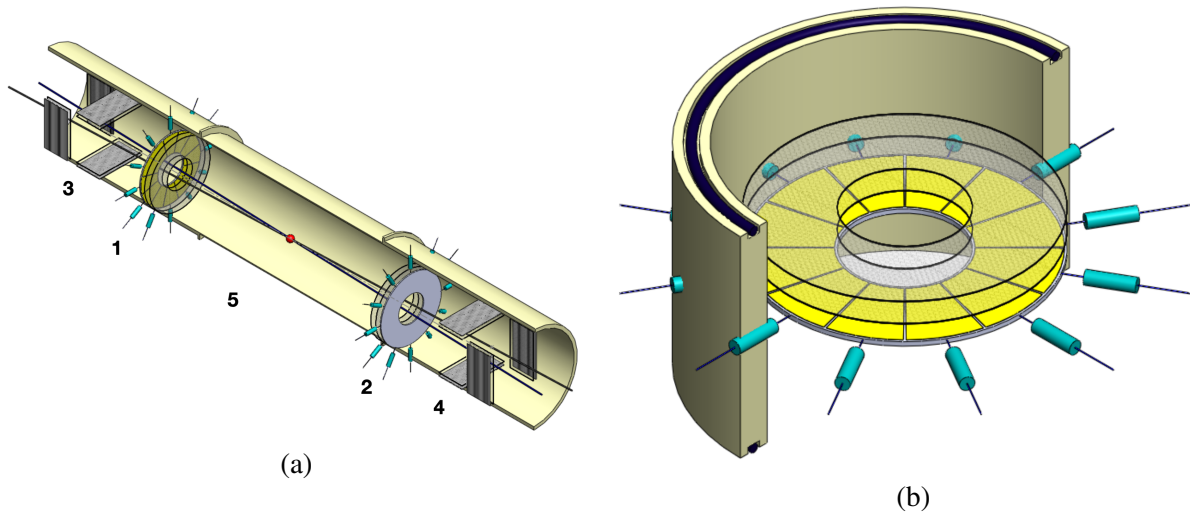
Figure 4.40: (a) Possible layout: the Fast Beam-Beam Collision (FBBC [423]) monitor composed of MCP discs (1 and 2) in combination with the Beam Position devices (BPM) (3 and 4) are situated symmetrically to the Interaction Point (5) inside the vacuum beam pipe of the NICA collider. (b) Compact module of the Fast Beam-Beam Collision Monitor (FBBC) based on circular MCPs. Sector cathode readout pads and two MCP setups are embedded into a separate flange with a hermetic 50- \Omega signal and HV feedthroughs (the latter are not shown).
