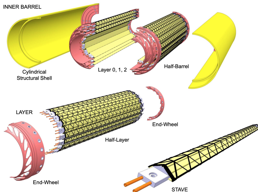
Figure 4.12: ALICE ITS2 Inner Barrel design [372].
