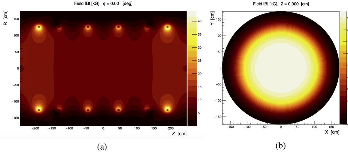
Figure 4.4: Magnetic field in the inner part of the SPD setup (a) z - r section; (b) x - y section at z = 0 .
