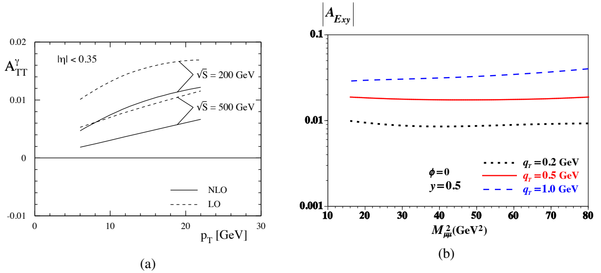
Figure 2.14: (a) A_{TT}^{\gamma} asymmetry for the prompt-photon production at 200 and 500 GeV coming from the q\bar{q} annihilation process calculated in LO [158] and NLO [159]. (b) Spin asymmetries |A_{E_{xy}}| for the proton-deuteron Drell-Yan process as a function of the dimuon mass squared for the dimuon rapidity y = 0.5 and different transverse momenta q_T [157].
