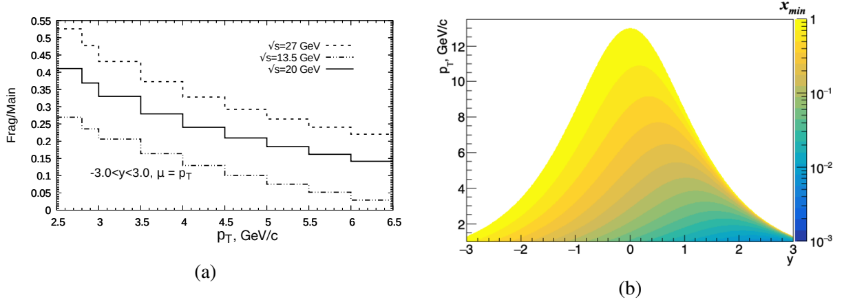
Figure 9.20: (a) Relative contribution of the fragmentation photons for the p - p collision energies \sqrt{s} = 13.5, 20 , and 27 GeV. (b) Minimal value of gluon x accessible via registration of prompt photon with rapidity y and transverse momentum p_T at \sqrt{s} = 27 GeV.
