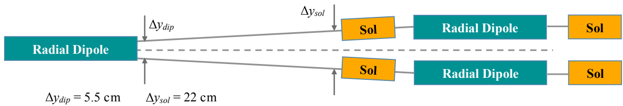
Figure 3.6: Placement of the SN solenoids in the vertical plane together with the radial dipoles.
