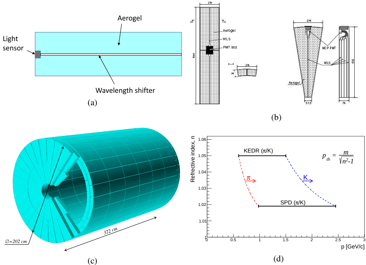
Figure 4.38: (a) Principle of ASHIPH operation. (b) KEDR aerogel counters: two barrel counters in a single housing (left), end-cap counter (right) [419]. (c) Possible arrangement of barrel and end-cap counters in SPD. (d) Momentum intervals of KEDR and SPD where the \pi/K separation is possible.
