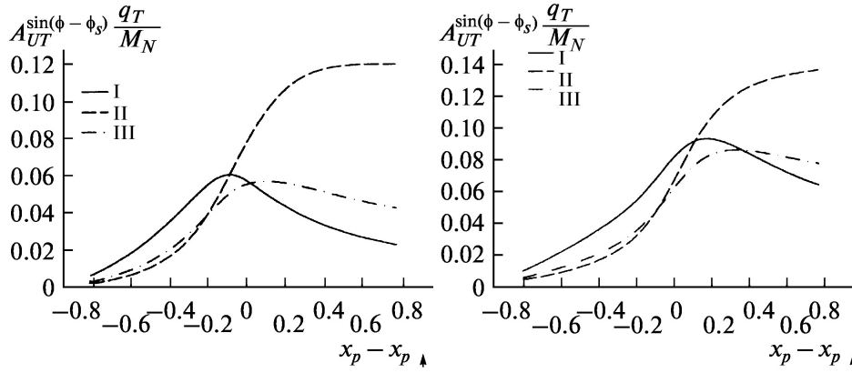
Figure 2.17: Estimated Sivvers asymmetries for the NICA conditions s = 20 GeV, Q^2 = 4 GeV 2 (left) and s = 20 GeV, Q^2 = 15 GeV 2 (right). Fits for the Sivvers functions are taken from [190].
