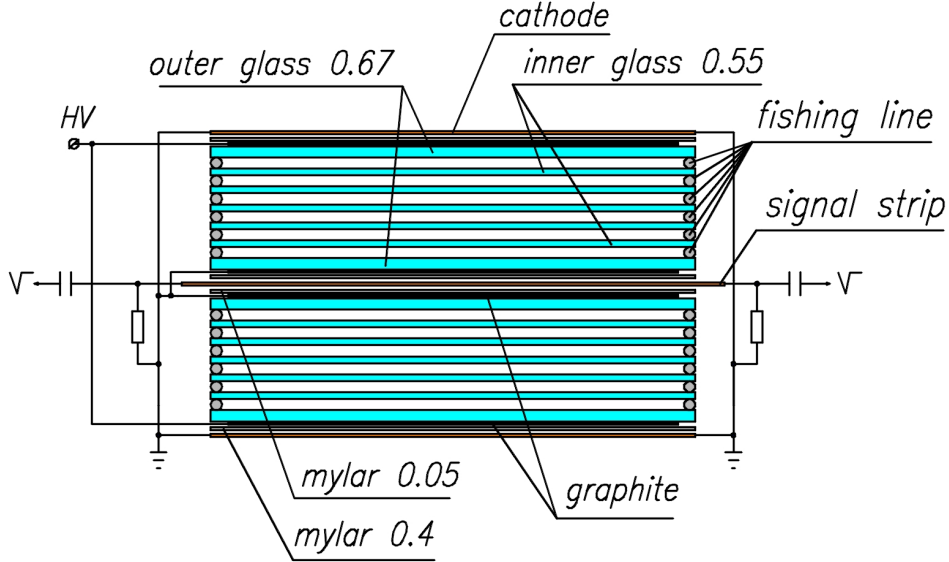
Figure 4.36: Schematic view of the twelve-gap mRPC [407].
