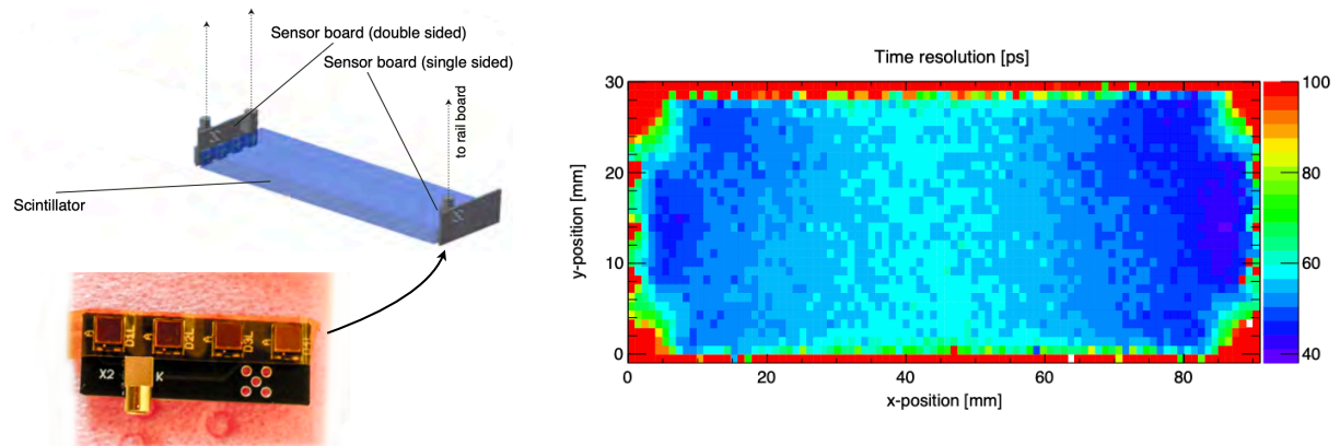
Figure 4.37: Left: schematic view to the plastic scintillator tile and a photo of the 4 SiPM board of PANDA [417]. Right: time resolution obtained from a position scan of a 90 \times 30 \times 5 \text{ mm}^3 EJ-232 scintillator tile read out by Hamamatsu SiPMs attached to opposite sides, 4 SiPMs in series per side [417].
