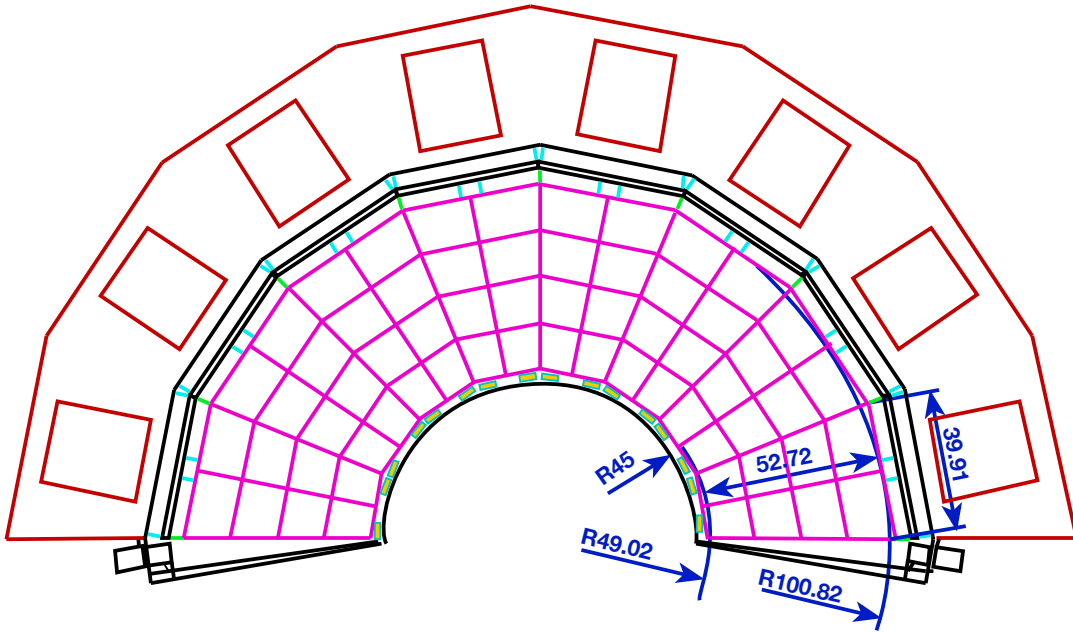
Figure 4.39: Beam-Beam Counter: azimuthal and polar angle segmentation [422]. All dimensions are in millimeters.
