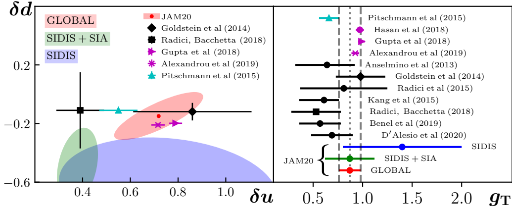
Figure 2.16: The results of the global analysis JAM20 (JAM collaboration) [184] along with others from phenomenology (black), lattice QCD (purple), and Dyson-Schwinger (cyan) for the tensor charges \delta u , \delta d and g_T = \delta u - \delta d at Q^2 = 4 \text{ (GeV/c)}^2 .
