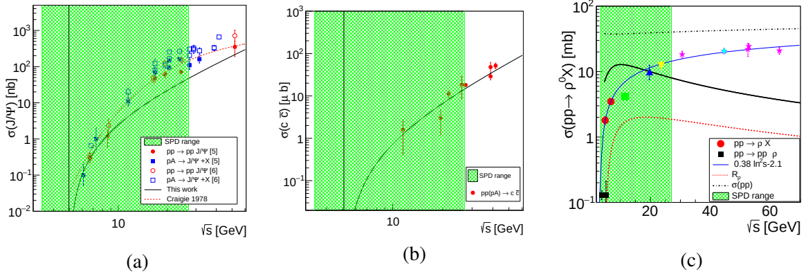
Figure 2.20: (a) Experimental data on J\psi production in p - p (red circles) and p - A (blue squares) reactions, from the recollections in Refs. [283] (filled symbols) and [284] (open symbols). The solid line is the calculation from Ref. [238]. (b) Total charm production in p - p and p - A collisions. The data are from Ref. [288]. The line is a threshold parametrization (see text). (c) Cross-section for \rho -meson production in p - p collisions: inclusive (different symbols and colors from different experiments) and exclusive data from pp \rightarrow pp\rho (black squares). The calculation from Ref. [289] shown as a black line. The red dashed line is the renormalization factor. The black dash-dotted line is the total pp cross-section. The first red point is the inclusive measurement from Ref. [290]. The blue line is the parametrization from Ref. [291]. The green filled region represents the SPD range.
