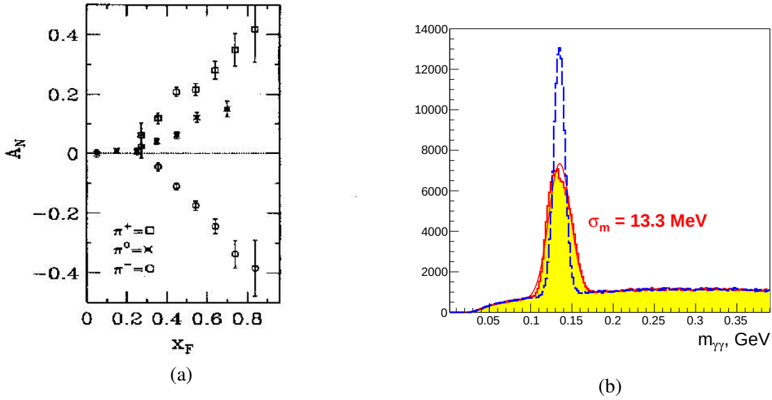
Figure 5.2: (a) Single transverse spin asymmetry A_N for inclusive pion production in p - p collisions at 200 GeV [175, 176]. (b) The \pi^0 reconstruction in the SPD ECal end-cup with (blue) and without (red) vertex position information.
