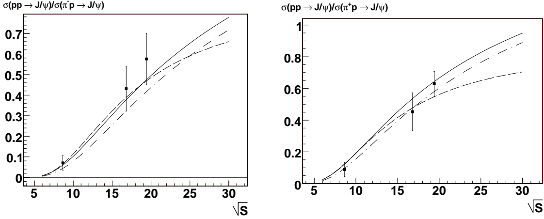
Figure 1: Ratios of cross-sections \sigma_{pp}/\sigma_{\pi^+p} on J/\psi production calculated with two models in comparison with the experimental data. Solid line corresponds to the “duality” model, Eqs. (4), (5). Dashed line corresponds to the “gluon evaporation” model, Eqs. (6), (7). Dot-dashed line corresponds to “gluon evaporation” model without gluon contribution. Here GRV94 [21] parametrization for the proton PDFs and GRV [20] parametrization for the pion PDFs are used. The experimental data (points with error bars) are taken from [9] (Tables 2 and 3).
