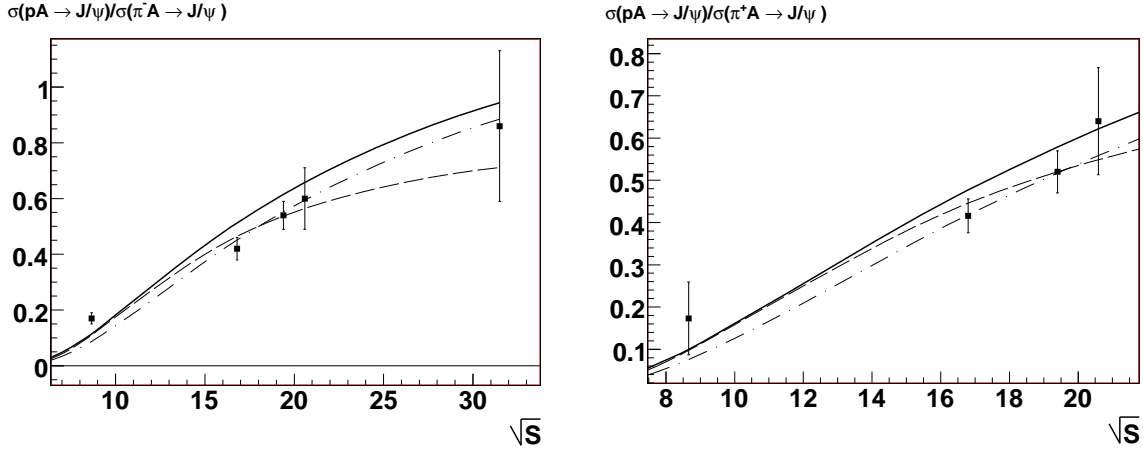
Figure 2: Ratios of cross-sections \sigma_{pA}/\sigma_{\pi^+A} on J/\psi production for the nuclear targets ( Z/A \simeq 0.4 ) calculated with two models in comparison with the experimental data. Solid line corresponds to the “duality” model, Eqs. (4), (5). Dashed line corresponds to the “gluon evaporation model”, Eqs. (6), (7). Dot-dashed line corresponds to the “gluon evaporation” model without gluon contributions. Here GRV94 [21] parametrization for proton PDFs and GRV [20] parametrization for pion PDFs are used. The points with error bars correspond to experimental data. First point: W, Z/A=0.40 [11]; second and third points: Pt, Z/A=0.40 [13]; fourth point: C, Z/A=0.5 [16]; fifth point: Be, Z/A=0.44 [14].
